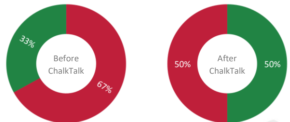
Science Benchmarks
