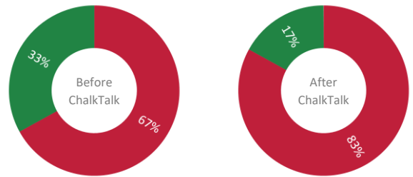
Reading Benchmarks
